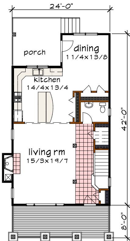
Floor 1 plan
