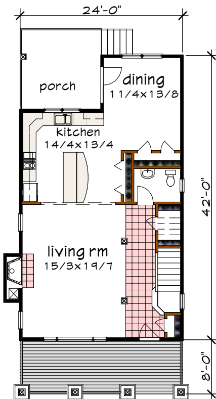
Floor 1 plan
