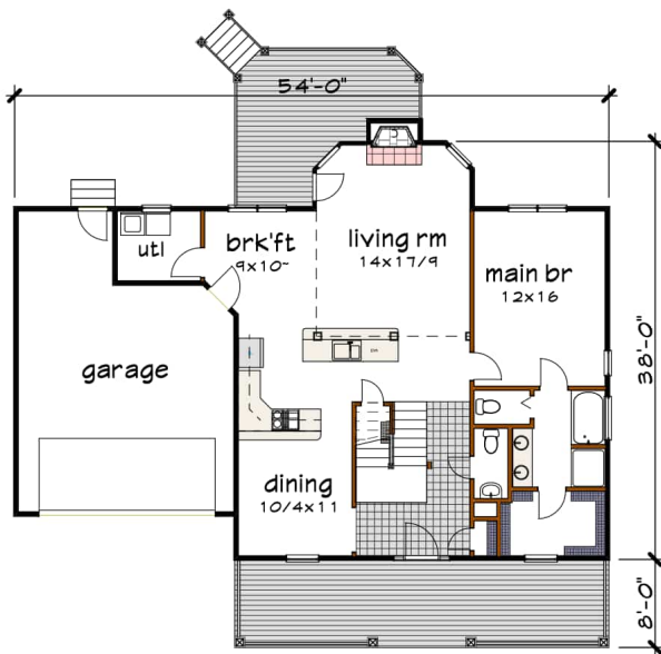
Floor 1 plan
