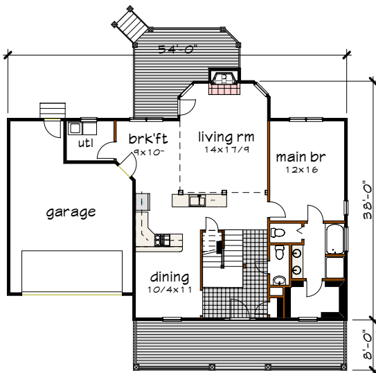
Floor 1 plan
