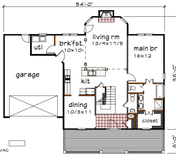
Floor 1 plan
