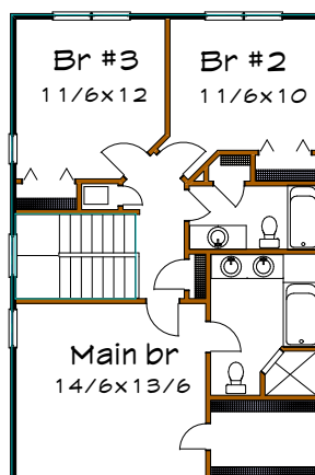
Floor 2 plan
