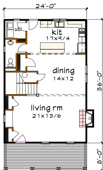
Floor 1 plan
