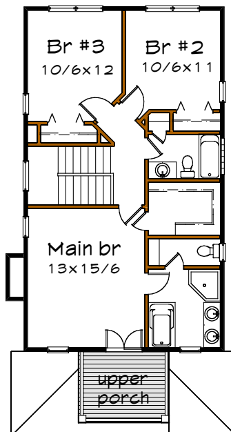
Floor 2 plan
