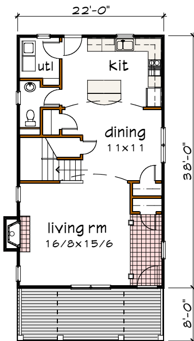
Floor 1 plan
