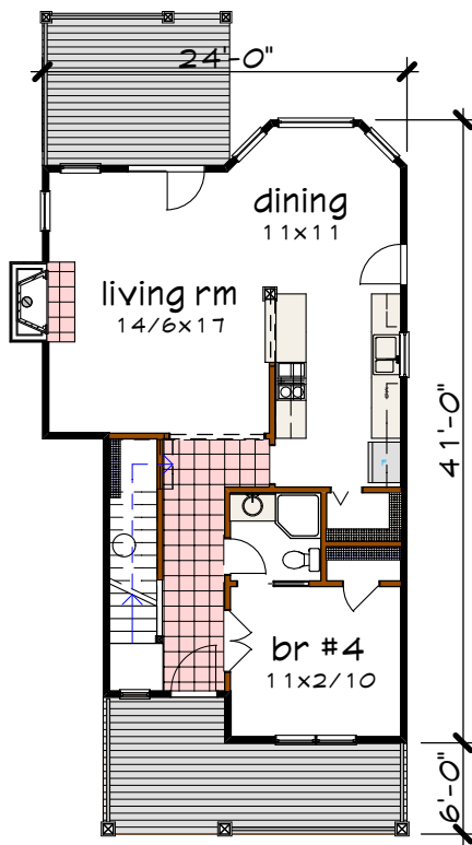
Floor 1 plan
