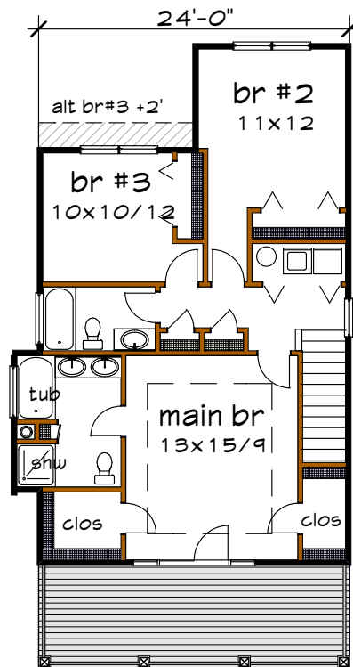
Floor 2 plan
