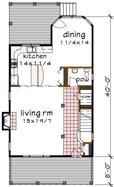
Floor 1 plan
