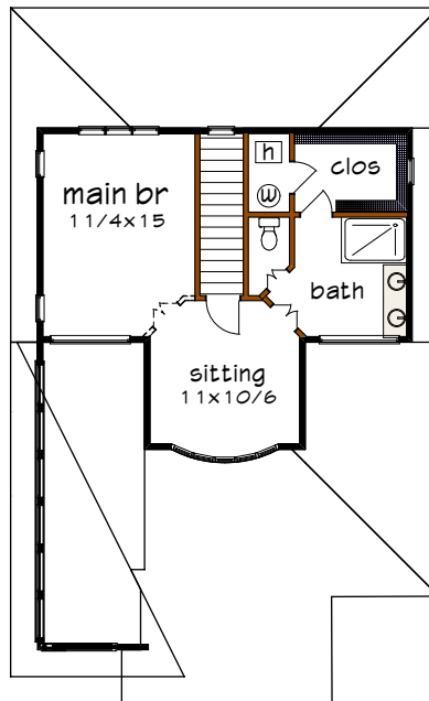
Floor 2 plan
