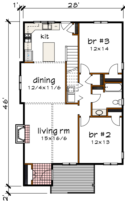
Floor 1 plan
