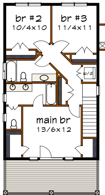
Floor 2 plan
