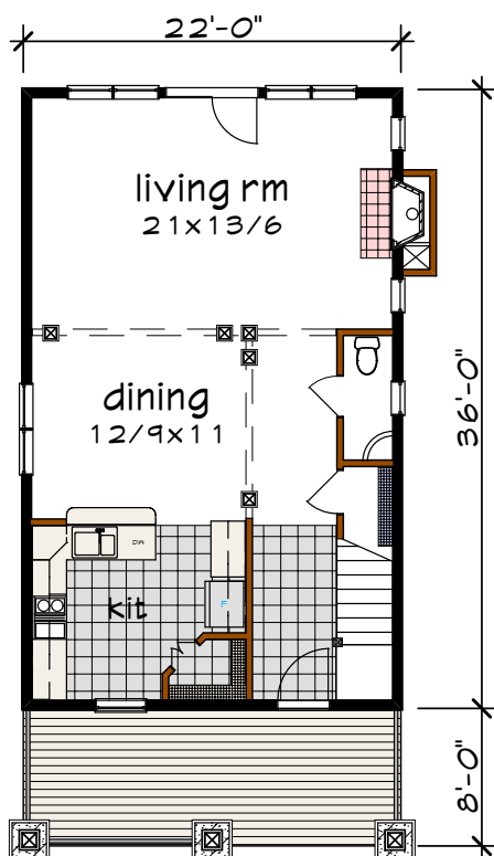
Floor 1 plan
