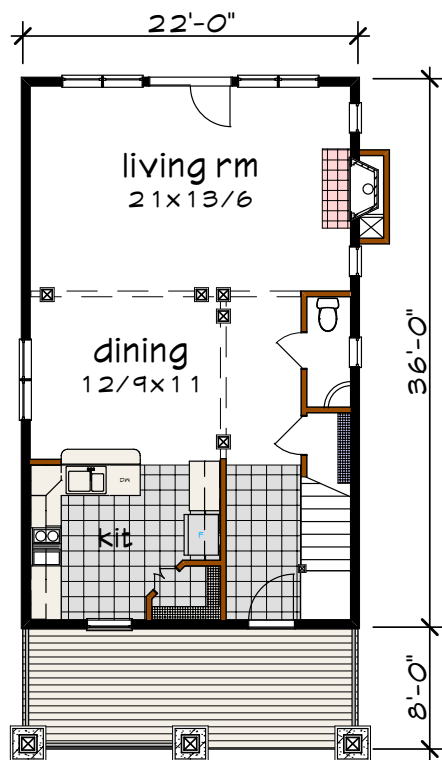
Floor 1 plan
