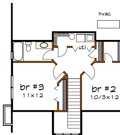
Floor 2 plan
