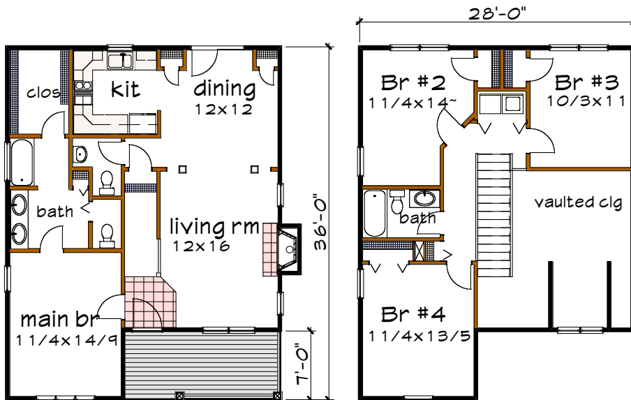
Floor 1 plan
