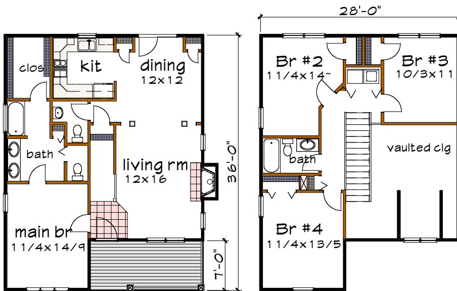
Floor 1 plan
