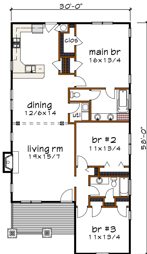
Floor plan
