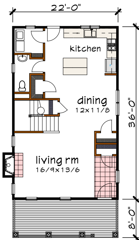
Floor 1 plan
