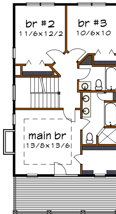
Floor 2 plan
