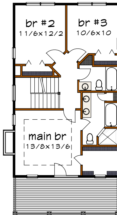
Floor 2 plan
