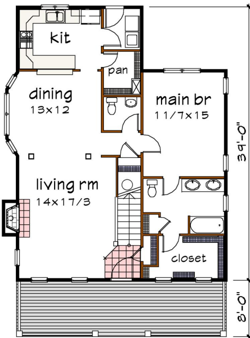
Floor 1 plan
