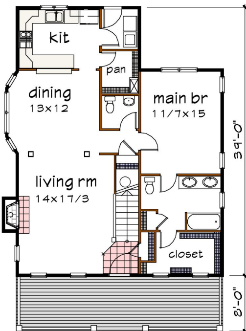
Floor 1 plan
