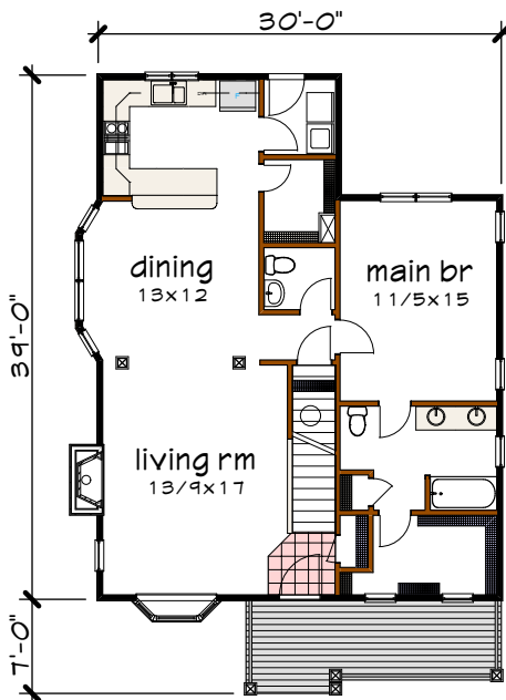
Floor 1 plan
