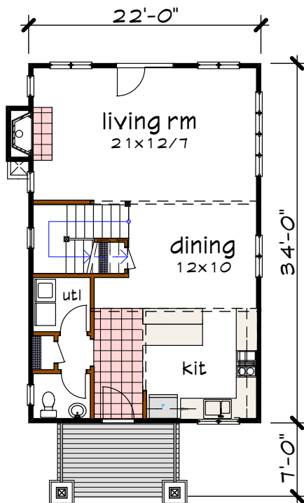
Floor 1 plan
