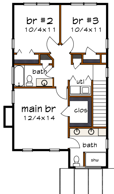
Floor 2 plan
