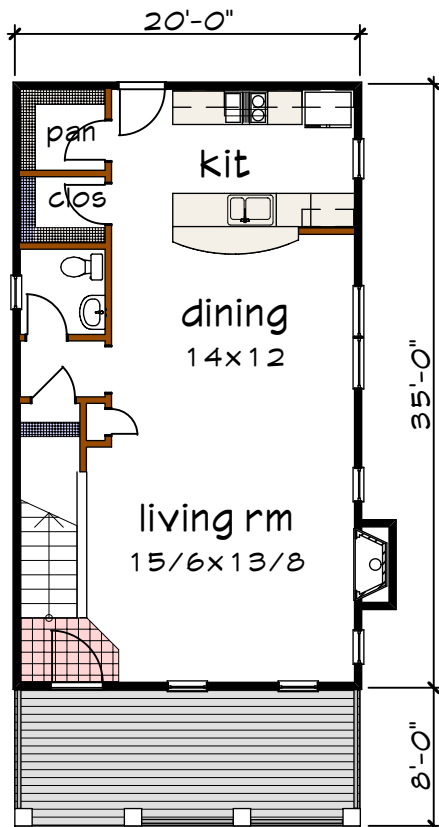
Floor 1 plan
