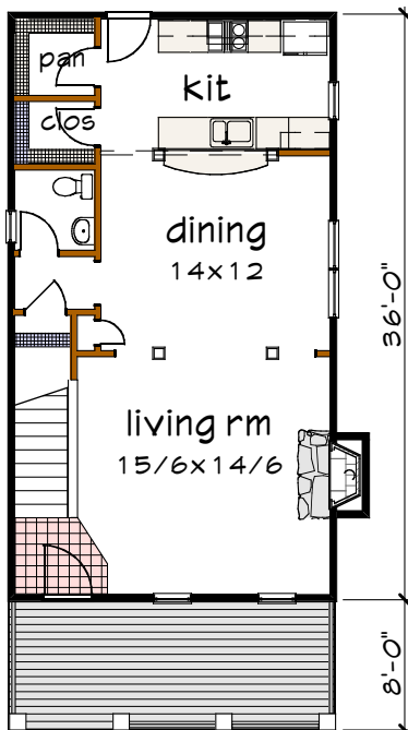
Floor 1 plan
