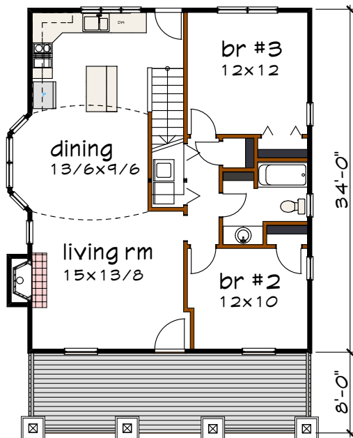
Floor 1 plan
