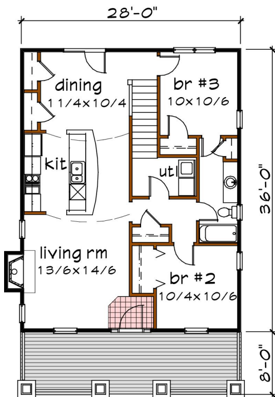
Floor 1 plan
