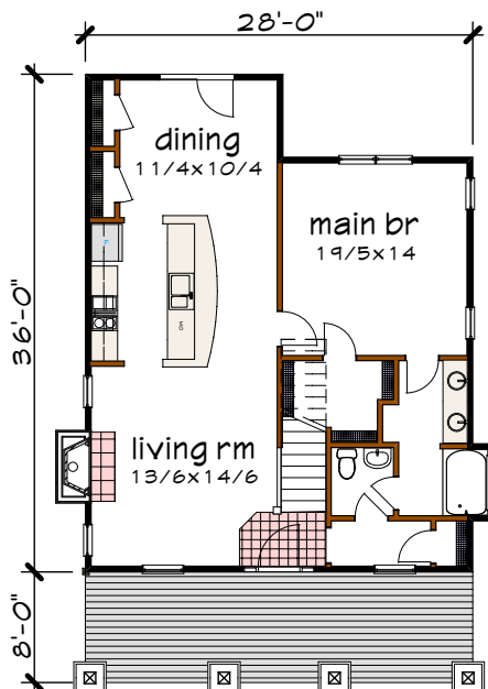
Floor 1 plan
