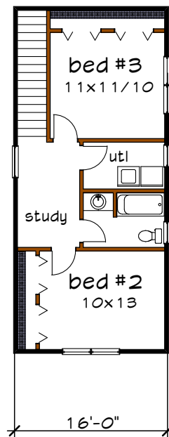
Floor 2 plan
