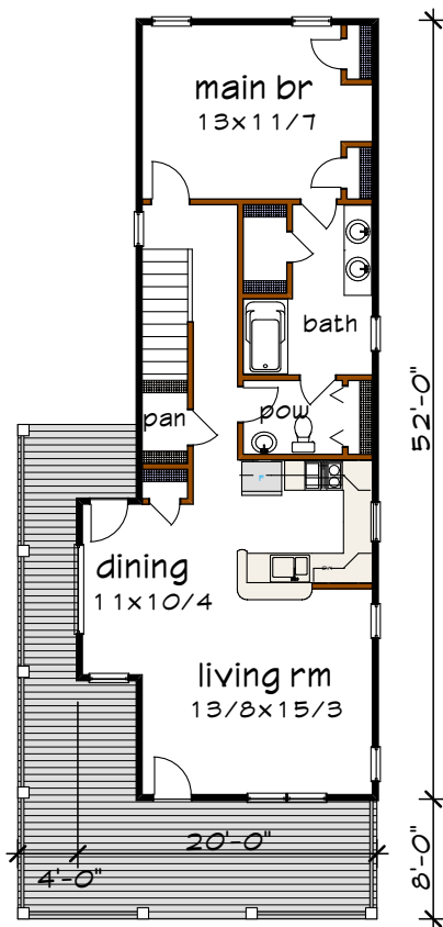
Floor 1 plan
