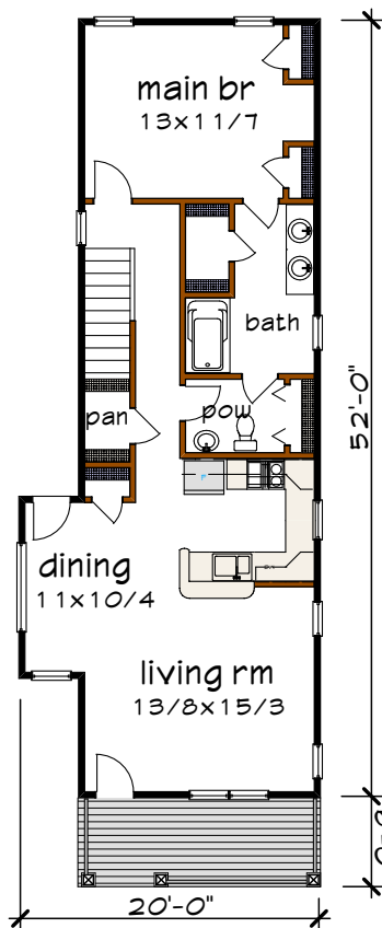
Floor 1 plan
