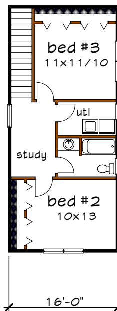
Floor 2 plan
