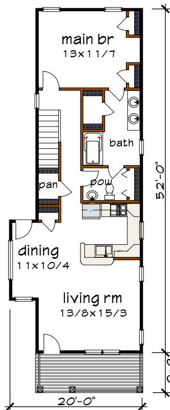
Floor 1 plan
