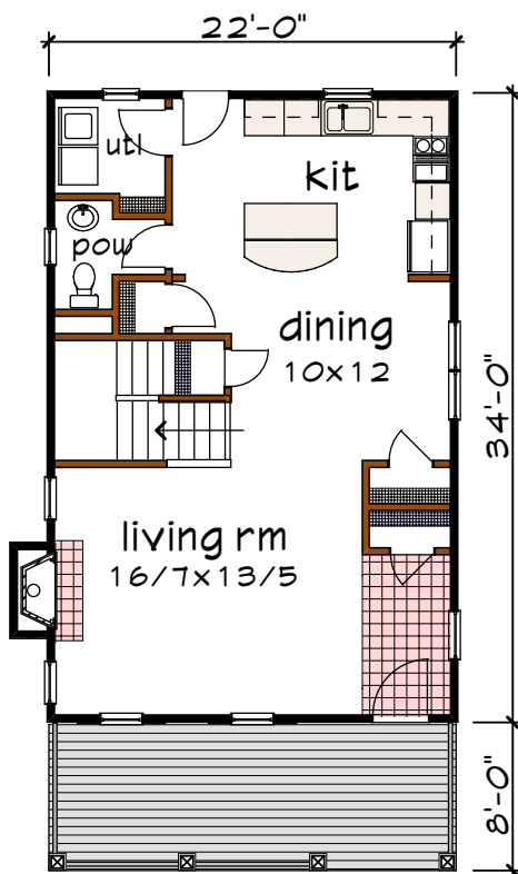
Floor 1 plan
