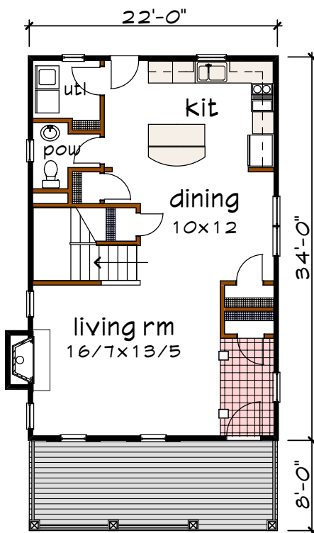
Floor 1 plan
