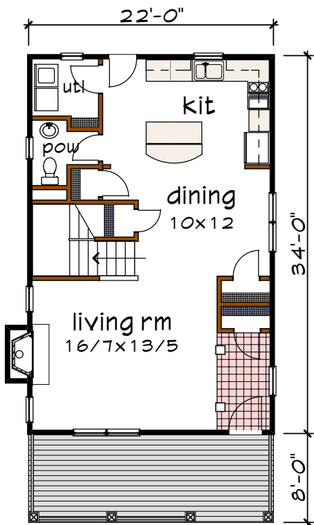
Floor 1 plan
