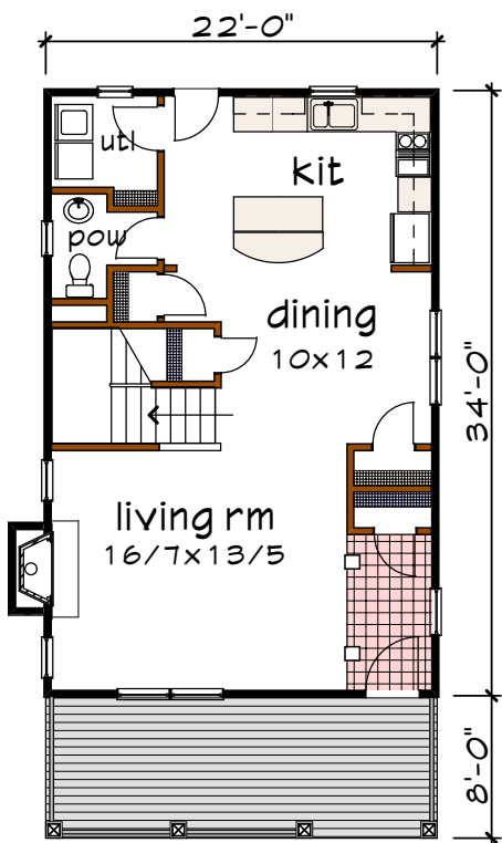
Floor 1 plan
