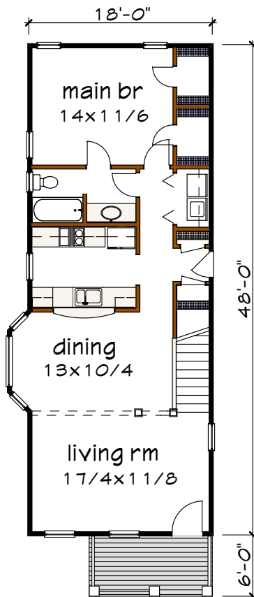
Floor 1 plan
