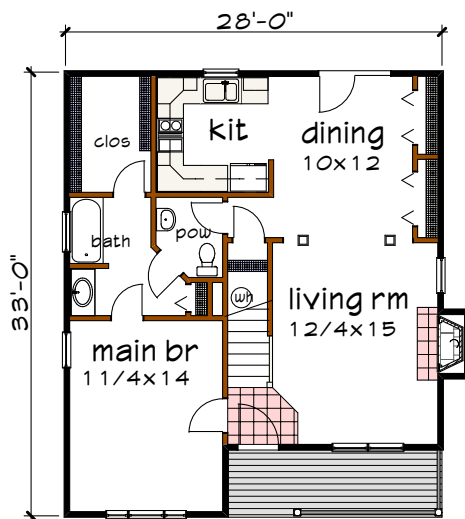
Floor 1 plan
