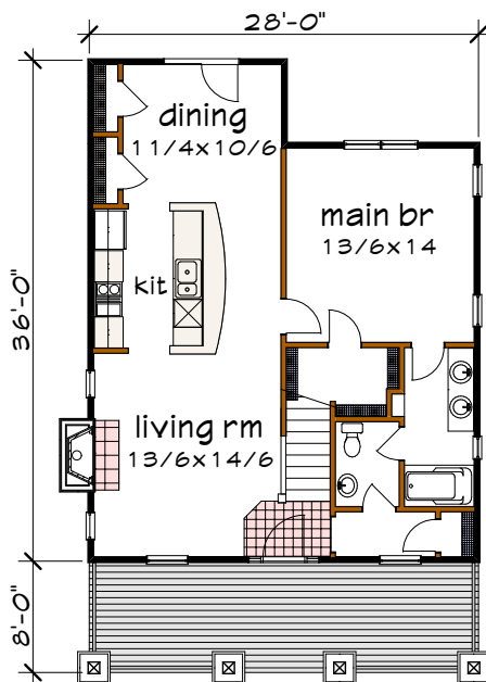
Floor 1 plan
