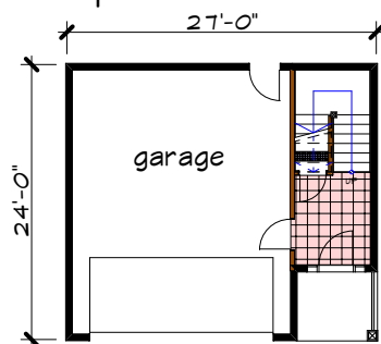
Floor 1 plan
