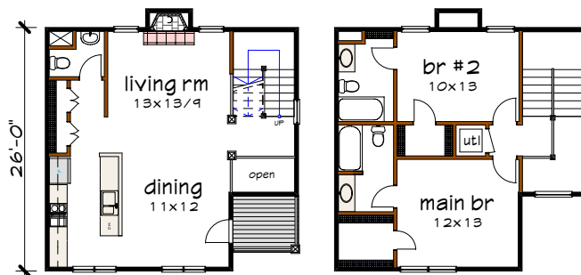
Floor 2 plan
