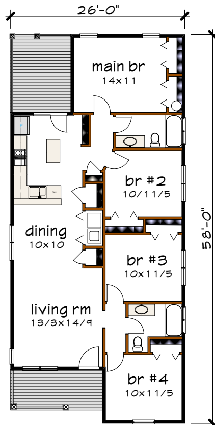
Floor 1 plan
