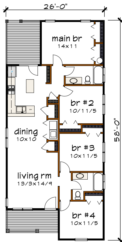
Floor 1 plan
