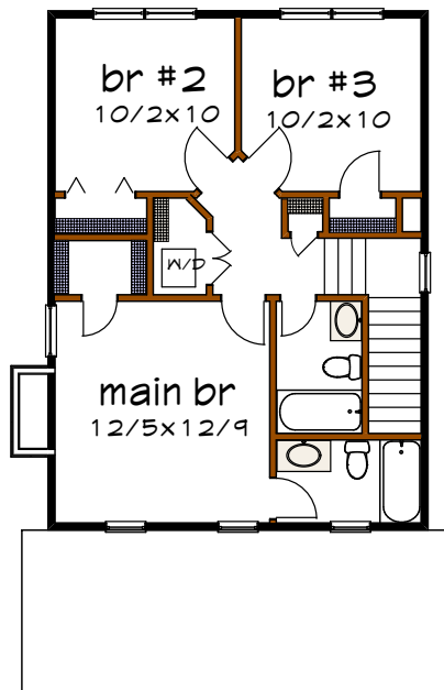
Floor 2 plan
