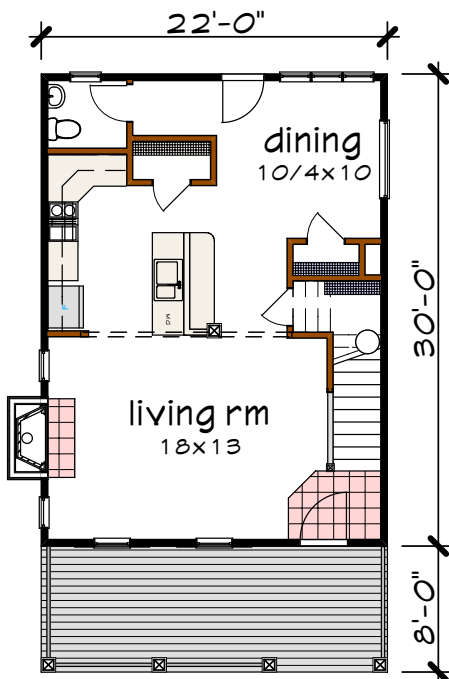
Floor 1 plan
