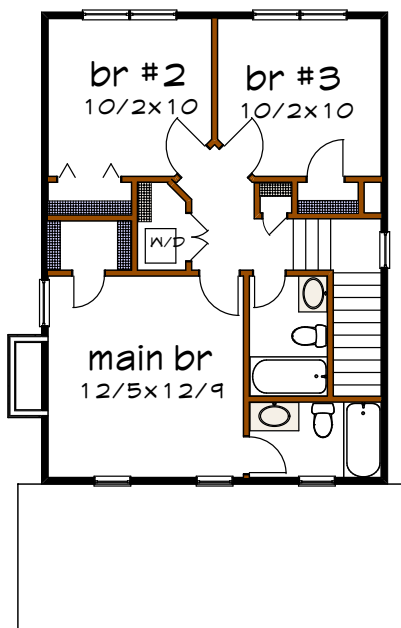
Floor 2 plan
