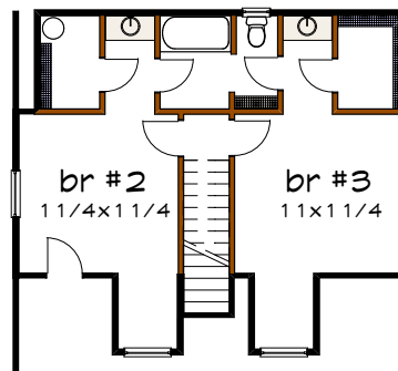
Floor 2 plan
