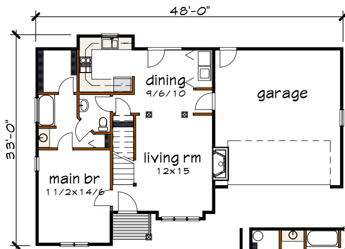
Floor 1 plan
