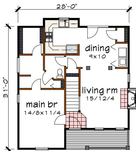
Floor 1 plan
