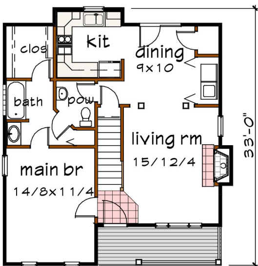
Floor 1 plan
