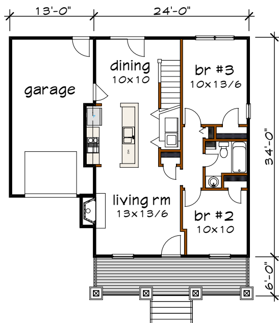
Floor 1 plan
