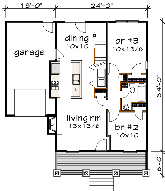
Floor 1 plan
